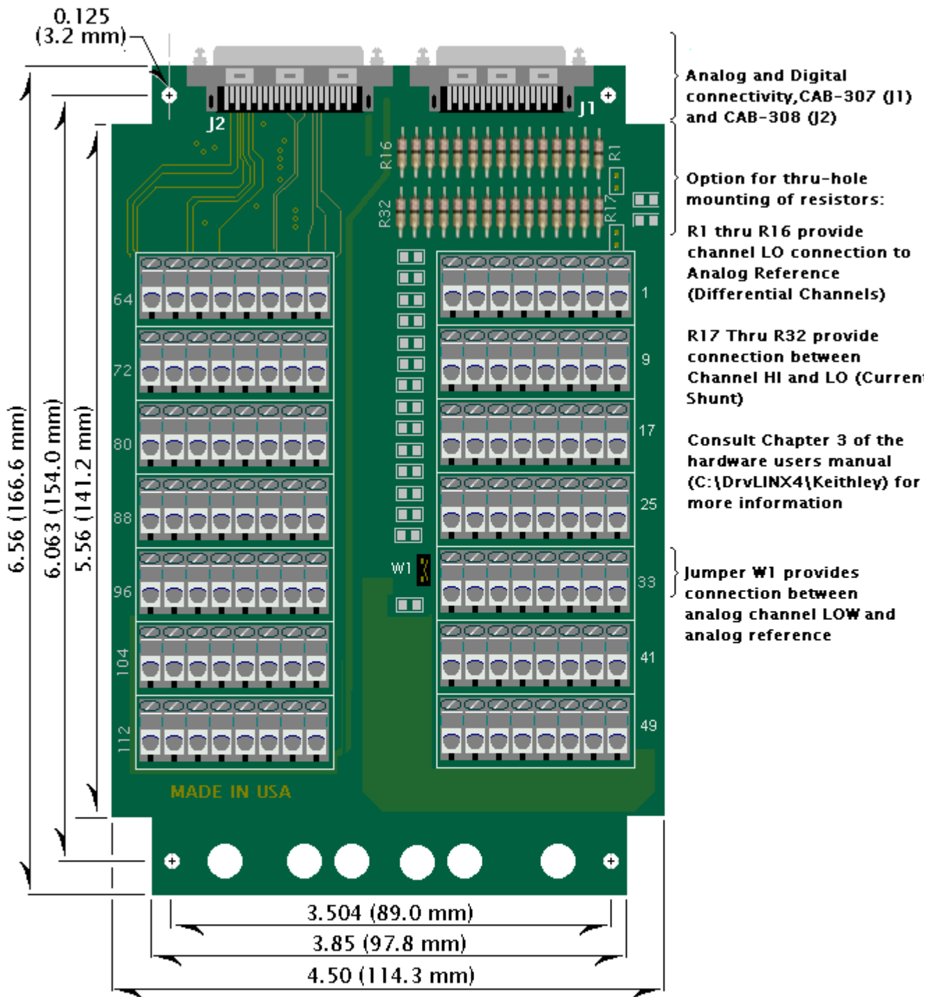
Attaching the STP-3110 screw terminal panel to the KPCI-3110 or KPCI-3116 board
