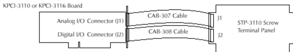
Attaching the STP-3110 screw terminal panel to the KPCI-3110 or KPCI-3116 board
